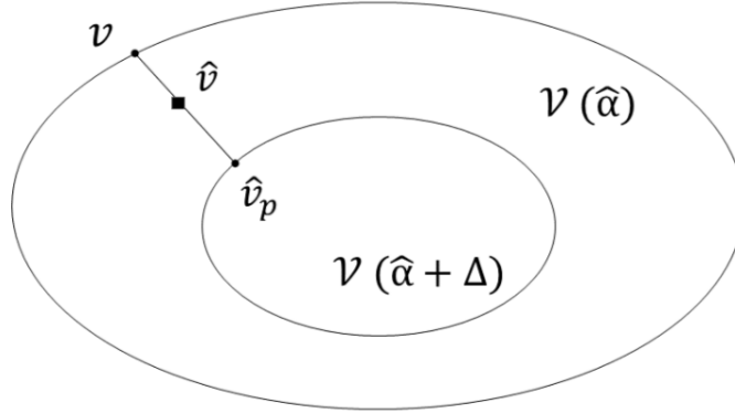
Figure 1: \hat{v} cannot be an interior point of \mathcal{V}(\hat{\alpha}) : otherwise, d(v, \mathcal{V}(\hat{\alpha} + \Delta)) = \|v - \hat{v}_p\| \geq \|v - \hat{v}\| \geq d(\hat{v}, \partial(\mathcal{V}(\hat{\alpha}))) \geq \epsilon , and d(v, \mathcal{V}(\hat{\alpha} + \Delta)) \leq \epsilon/2 (contradiction).
