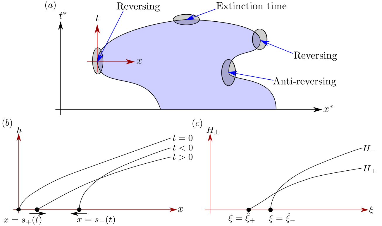
Figure 1: Panel (a): Schematic scenario of one possible evolution of the compact support (blue region) of a solution to (1.1). Regions in the (x^*, t^*) -plane corresponding to extinction time, reversing and anti-reversing events are highlighted. Panel (b): Possible snapshots of the profile of h(x, t) (in the local (x, t) -coordinate system highlighted in red in panel (a)) at three different times local to the reversing event. Panel (c): The corresponding solution profiles H_{\pm} in the self-similar coordinate system defined in (1.4).
