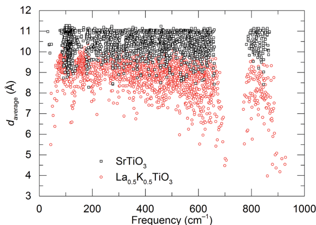
Fig. 1 Phonon localisation in \text{La}_{0.5}\text{K}_{0.5}\text{TiO}_3 (red circles) determined from DFT calculations compared against interactions in the perovskite \text{SrTiO}_3 (black squares). The parameter d_{\text{average}} is calculated for individual phonon modes as the mean distance between the ten atoms that participate to the greatest extent in that phonon mode as defined by their displacement amplitudes.
