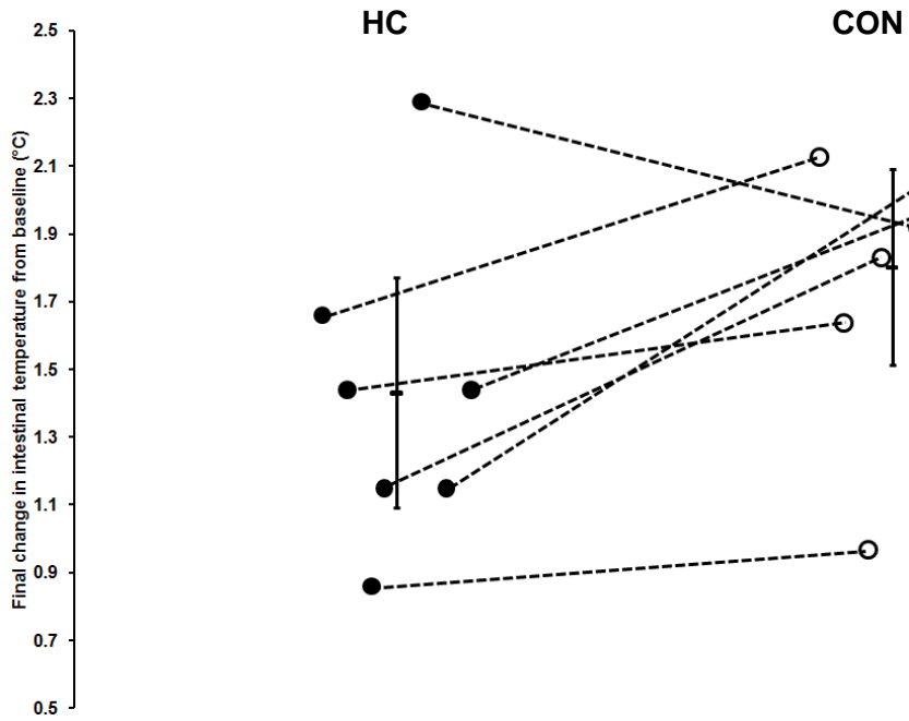
Figure 49: Individual data points demonstrating final change in intestinal temperature Error bars and black horizontal line represent 90% confidence intervals and the mean, respectively. Closed circles represent hand cooling trials, open circles represent control trials.
