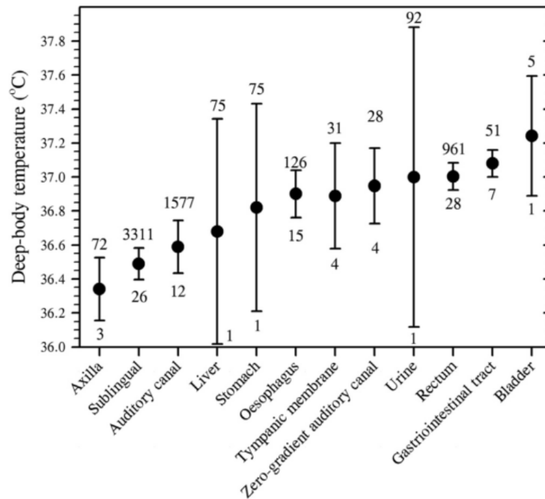
Figure 1: Variances in resting body temperature
