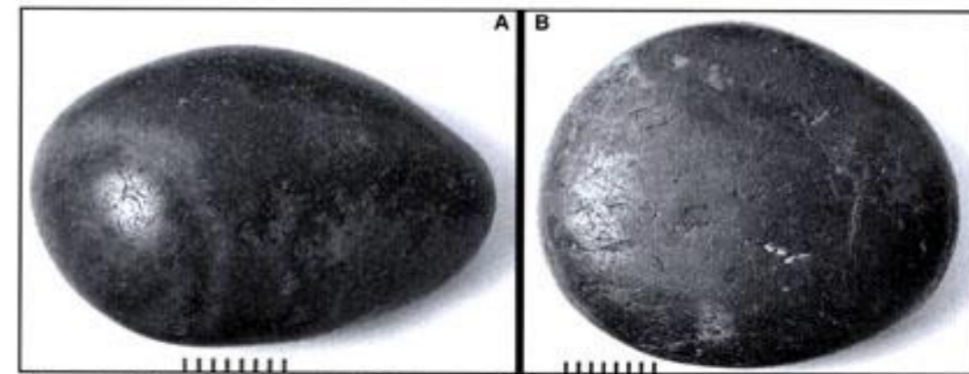
Figure 3. A. Example of conchoidal fractures visible on the surface of a chert gastrolith collected from elasmosaur remains (KUVV 1318) from the Greenhorn Limestone, Ellsworth County, KS; B. Conchoidal fractures on the surface of a probable gastrolith (FHSV VP-15719) from the Kiowa Shale of Kiowa County, KS (scale = mm).
