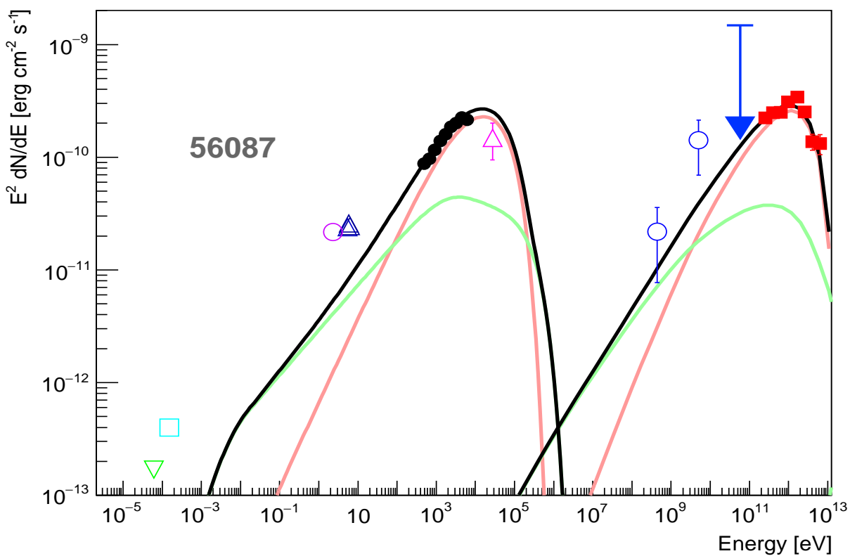
Fig. 7. Broadband SED for MJD 56087 (VHE flare from 2012 June 9), fitted with a one-zone SSC model (top) and a two-zone SSC model (bottom). See Figure 5 for explanation of markers and other details. In the bottom panel, the green line depicts the emission of the first (large) zone responsible for the baseline emission, and the red line the emission from the second (smaller) zone, that is responsible for the flaring state. The fit results from the one-zone SSC model fit are reported in Table 2, while those from the two-zone SSC model fit are reported in Table 3.
