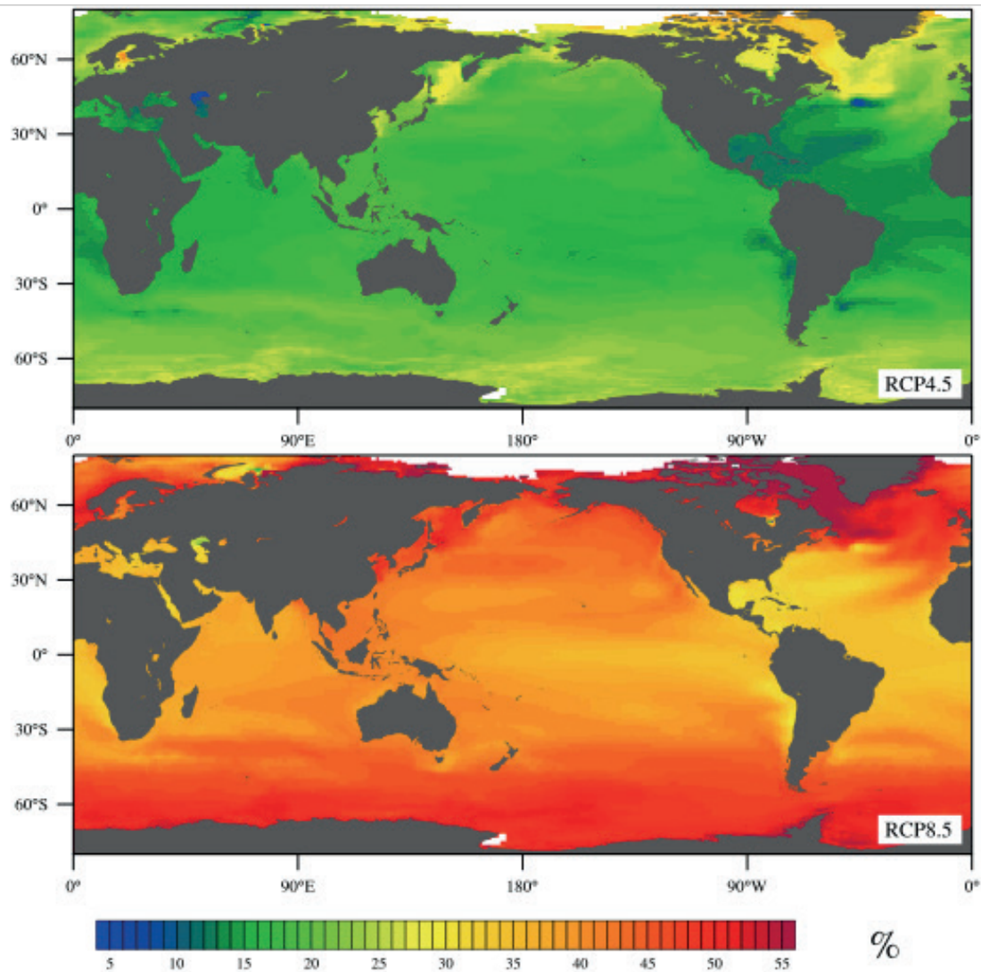
Projected percent change in aragonite saturation state (an ocean acidification indicator) in by 2100 under ‘Moderate Mitigation’ (top) and ‘Business as Usual’ (bottom) scenarios.
