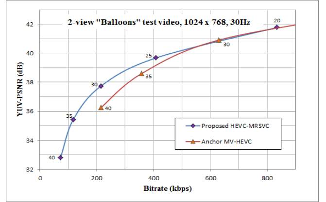
FIGURE 10. YUV-PSNR for MV-HEVC anchor and the proposed HEVC-MRSVC codecs for coding "Balloons" stereo test videos at different bitrates.
