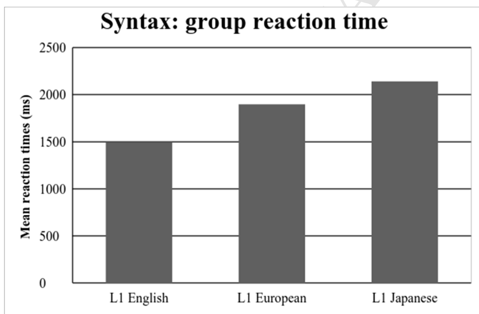
Figure 4: Reaction time for syntactic judgements (y-axis) and L1 group (x-axis)
