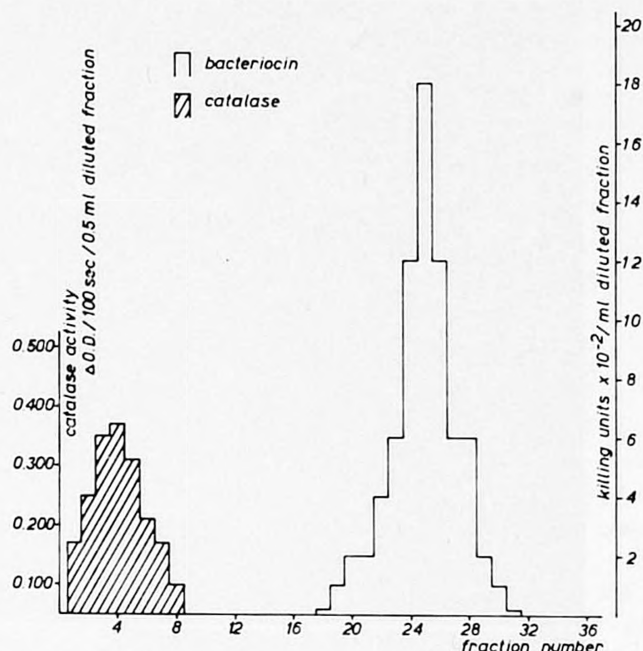
FIG. 3. Centrifugation of a mixture of partially purified bacteriocin (fraction 2 after gel filtration) and catalase on a linear sucrose-gradient (5 to 20% sucrose in 0.05 \text{ M} Tris buffer, pH 7.0).
