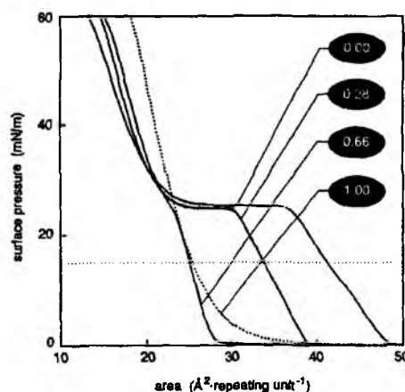
Fig. 1. Surface pressure–area isotherms of mixtures of 3 and AB. The base mole fraction of 3 is indicated. The temperature was 15^\circ\text{C} and the speed of compression was 5 \text{ \AA}^2 \text{ min}^{-1} per repeating unit.
