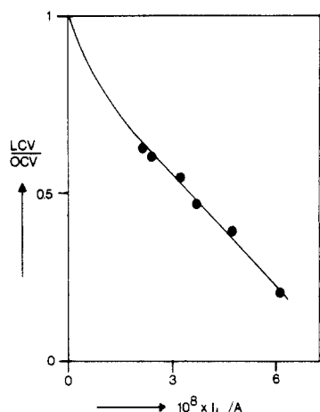
Figure 7. Normalized load-circuit voltages vs load currents for a concentration cell with a sodium picrate-1c complex as membrane; T = 80\text{ }^{\circ}\text{C} .
