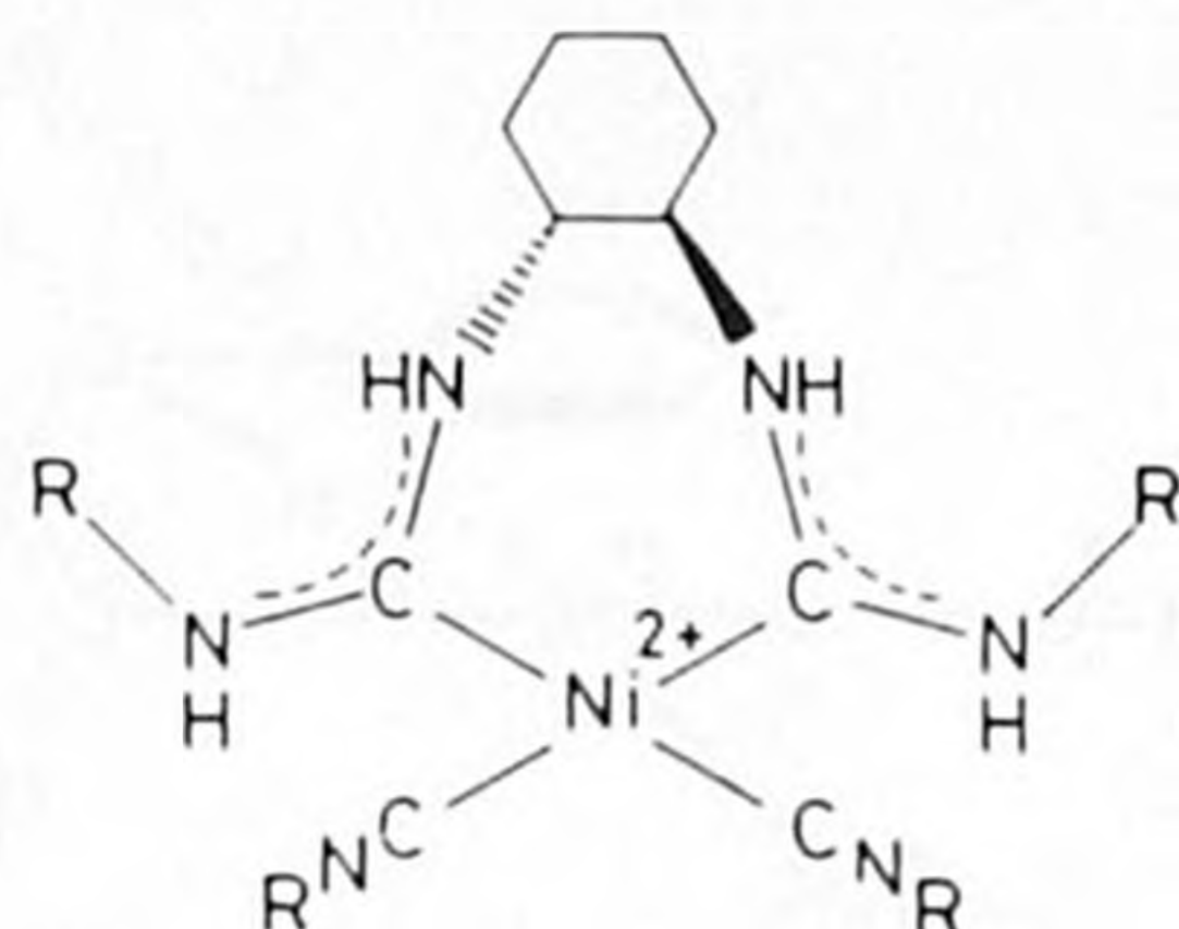
Figure 5. Starting complex for the polymerization of isocyanides with ( R,R )-1,2-diaminocyclohexane as the initiator.
