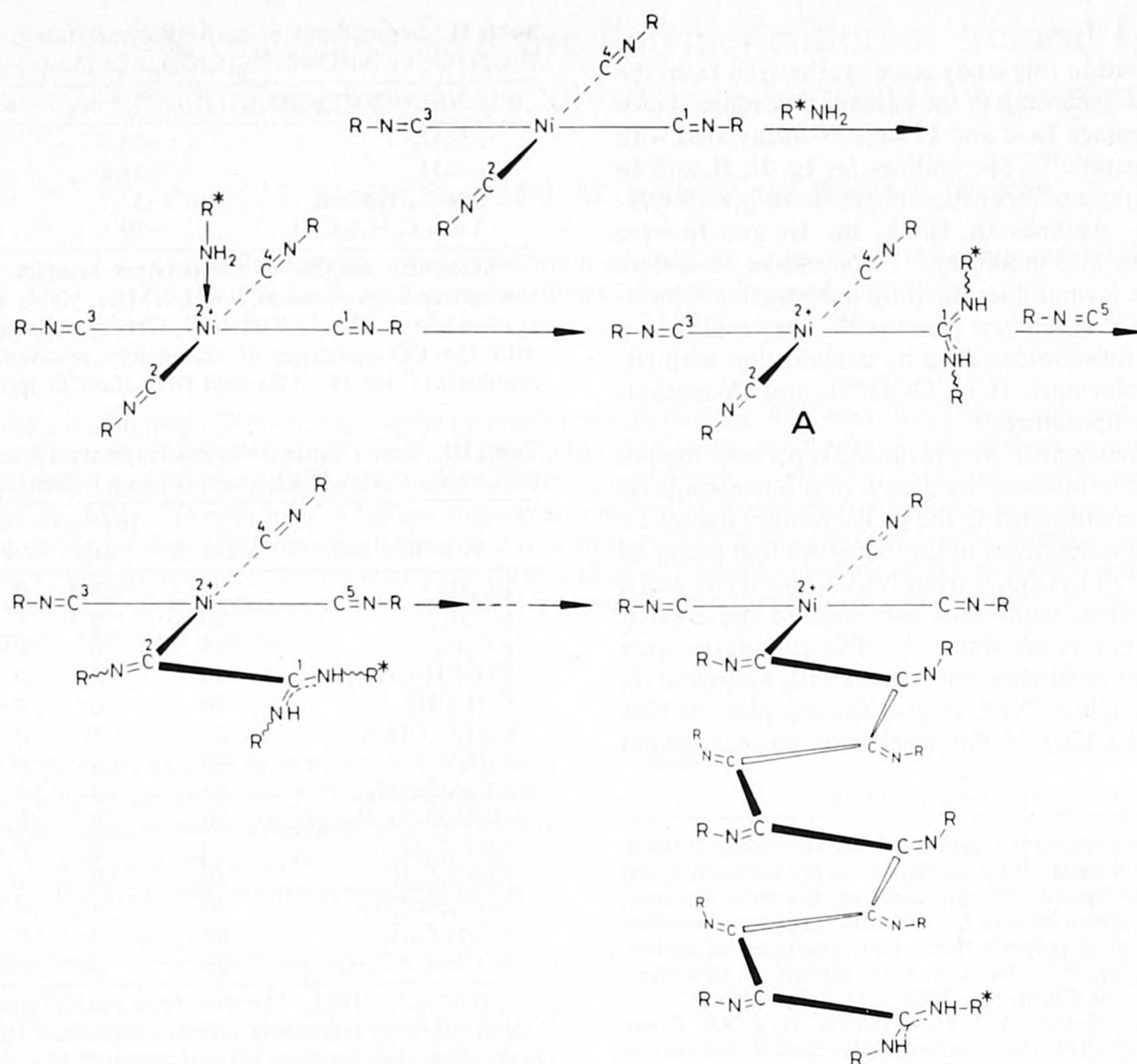
Figure 1. Mechanism of polymerization of isocyanides.
