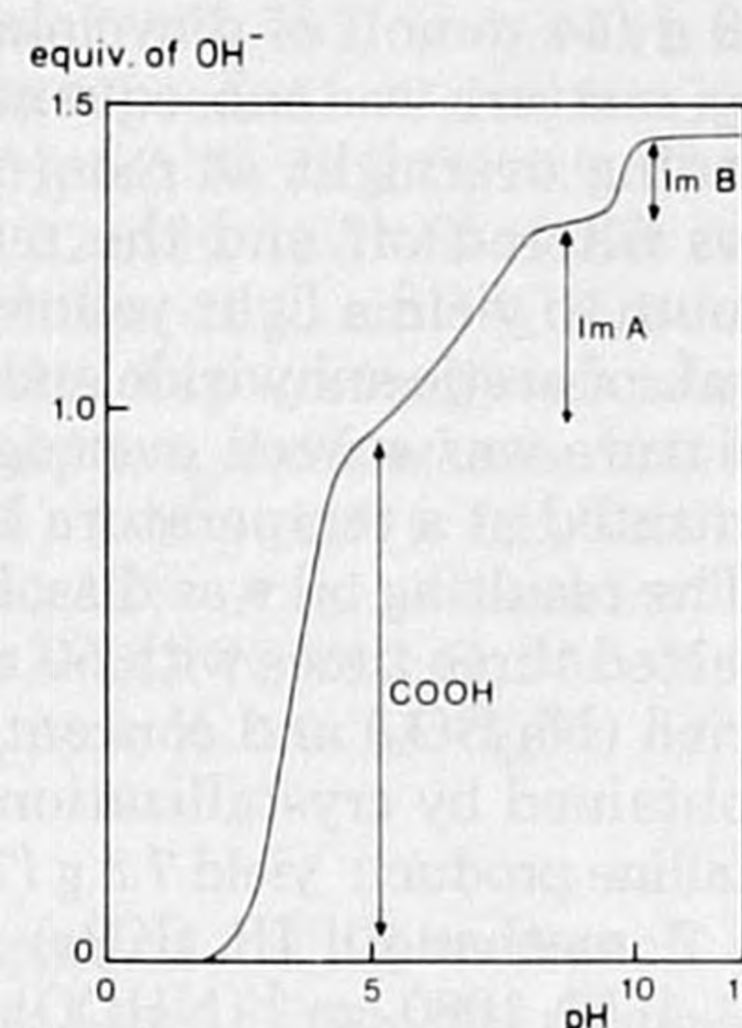
Figure 4. Titration curve of copolymer 11dp.
