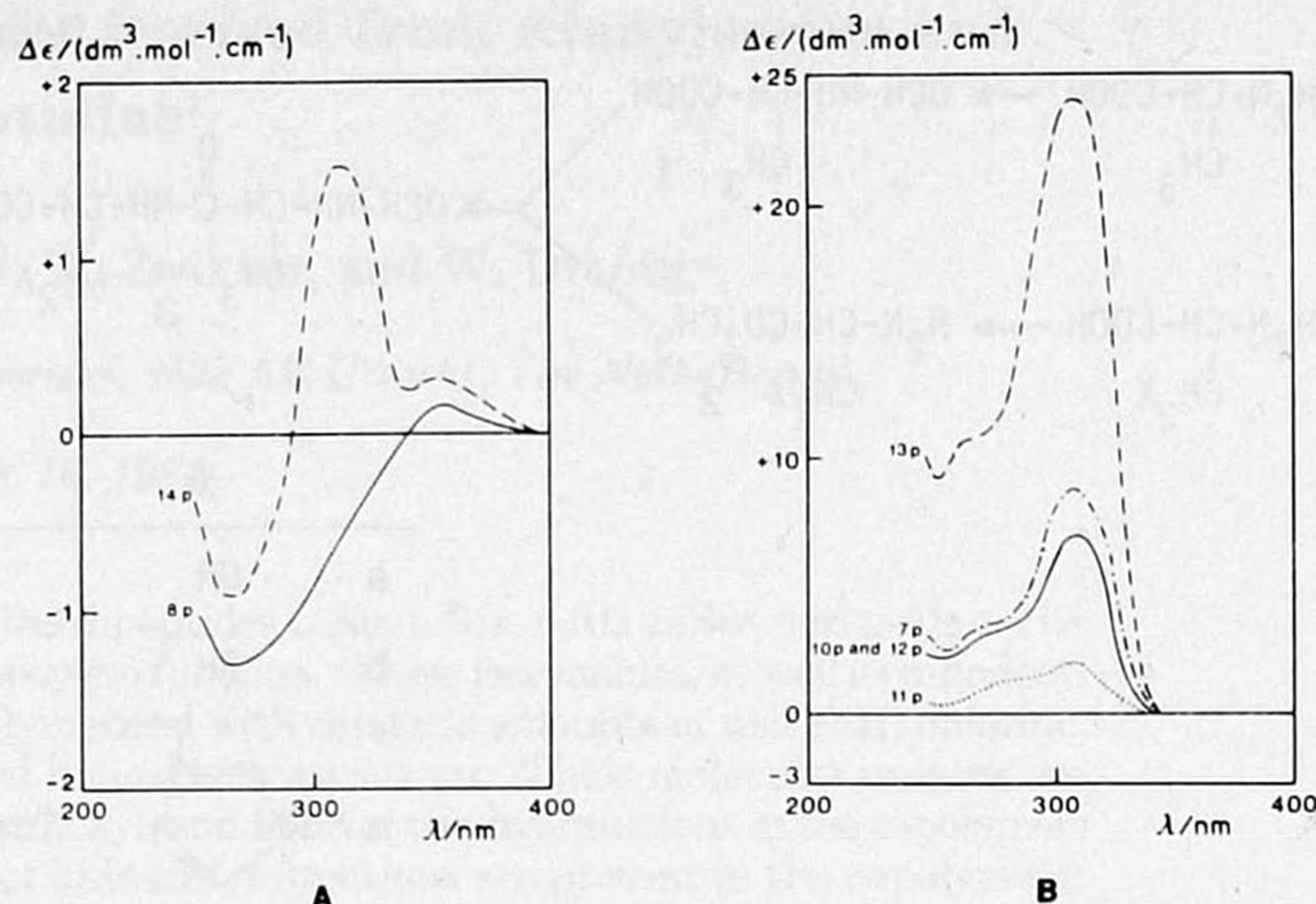
Figure 2. (A). CD spectra of homopolymer 8p and copolymer 14p in chloroform-methanol, 5:2 v/v. (B). CD spectra of homopolymer 7p and copolymers 10p-13p in chloroform-methanol, 5:2 v/v.
