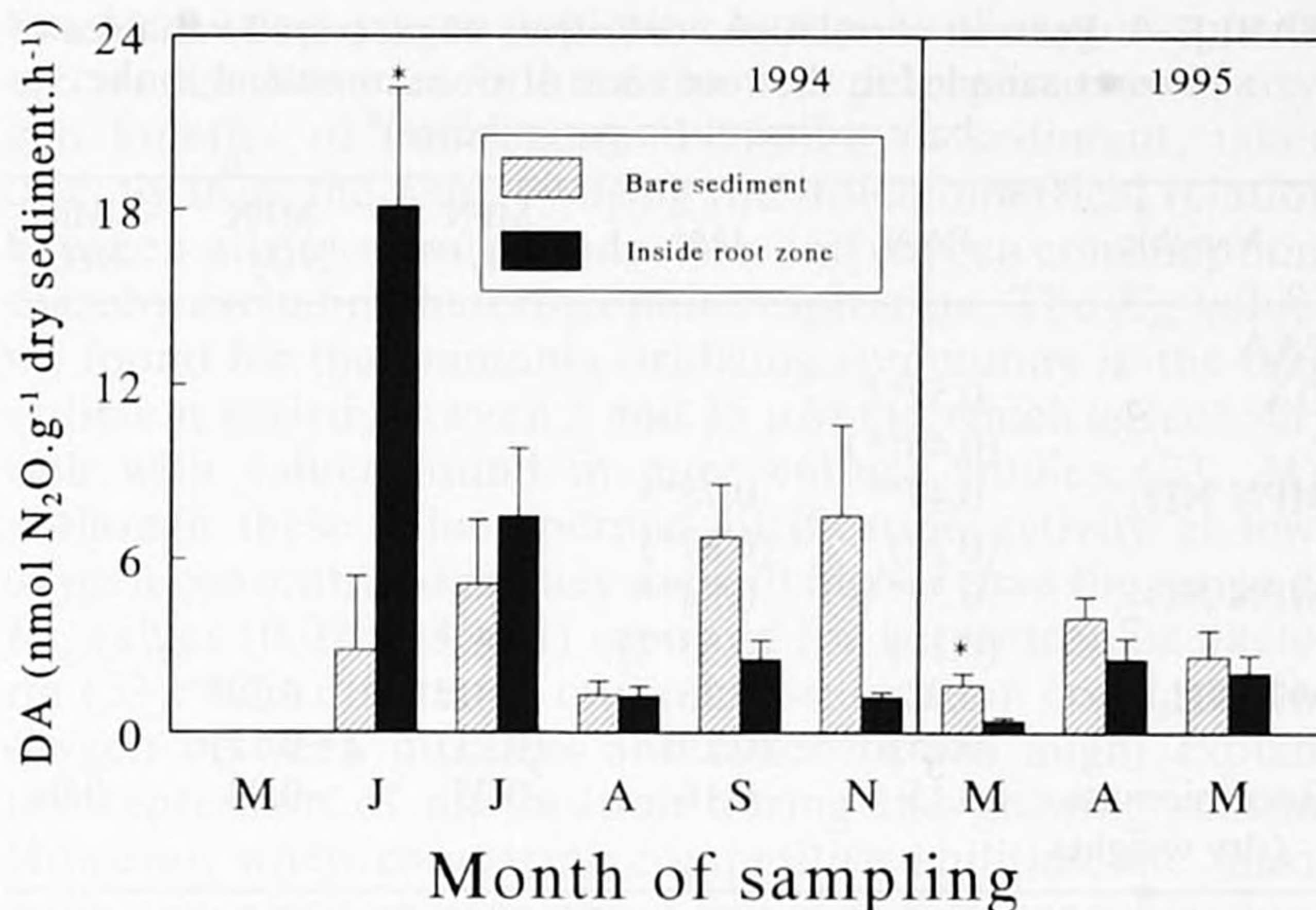
FIG. 4. Denitrification activities (DA) in slurries from sediment cores sampled in the root zone of G. maxima and the bare sediment at Lake Drontermeer in 1994 and 1995. Bars represent means ( \pm standard errors) of 5 replicate cores. Significant differences between activities in the root zone and the bare sediment are indicated by asterisks (two-sample t test, n = 5 ). **, P < 0.01 ; *, P < 0.05 .
