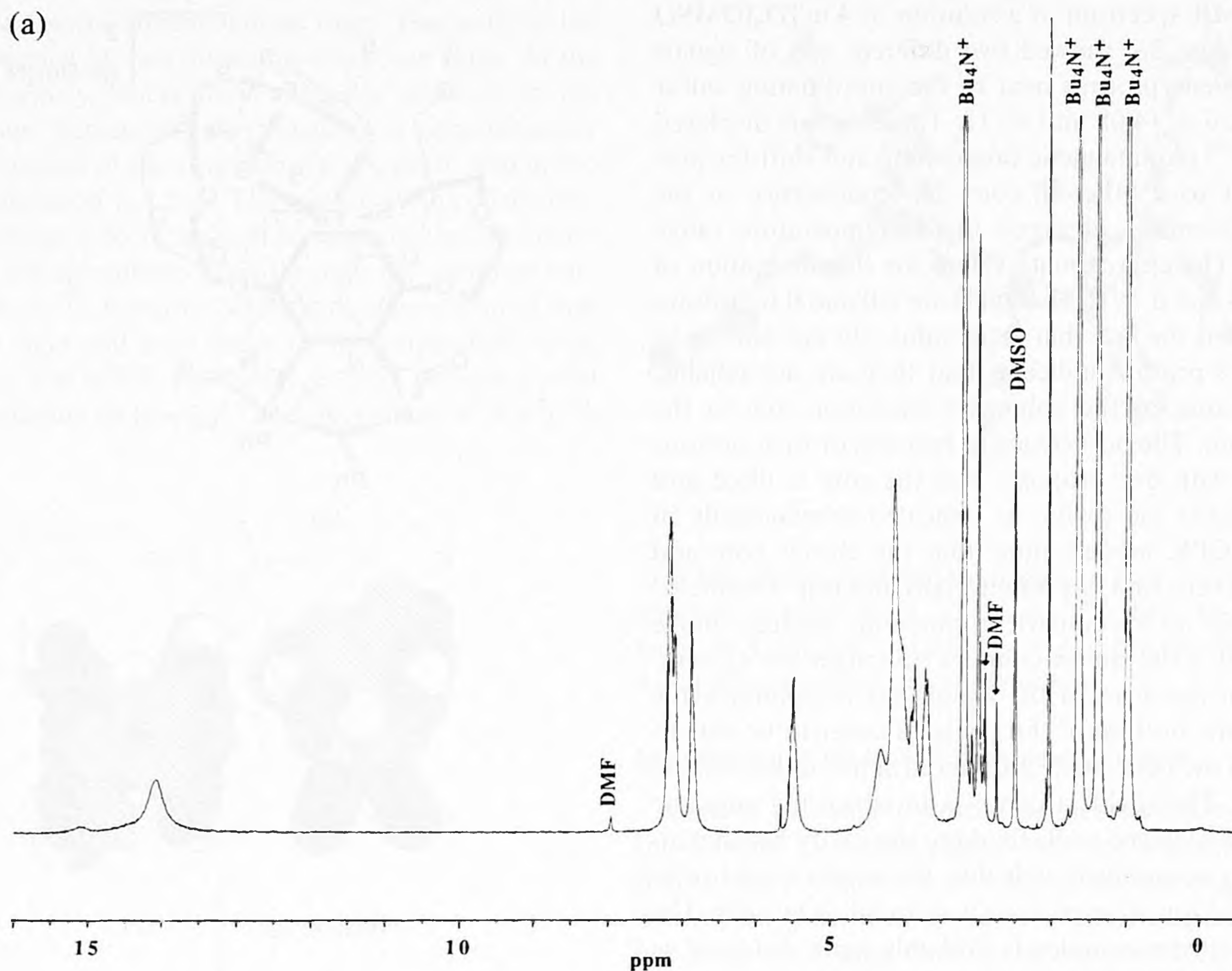
Figure 3. (a) and (b) 400-MHz ^1\text{H} - and ^{13}\text{C} -NMR spectra, respectively, of 4 in DMSO; (c) temperature dependence of the isotropic shift of each of the \text{CH}_2\text{S} protons in 4 (solvent [\text{D}_6]\text{DMSO} )
