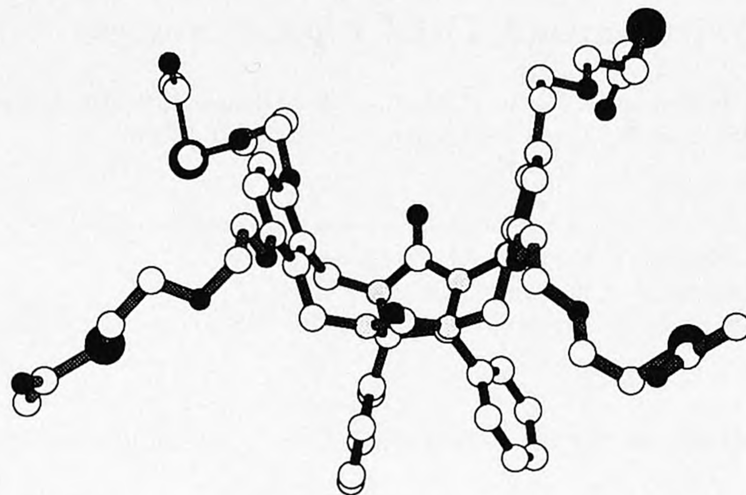
Figure 1. X-ray structure of 2
