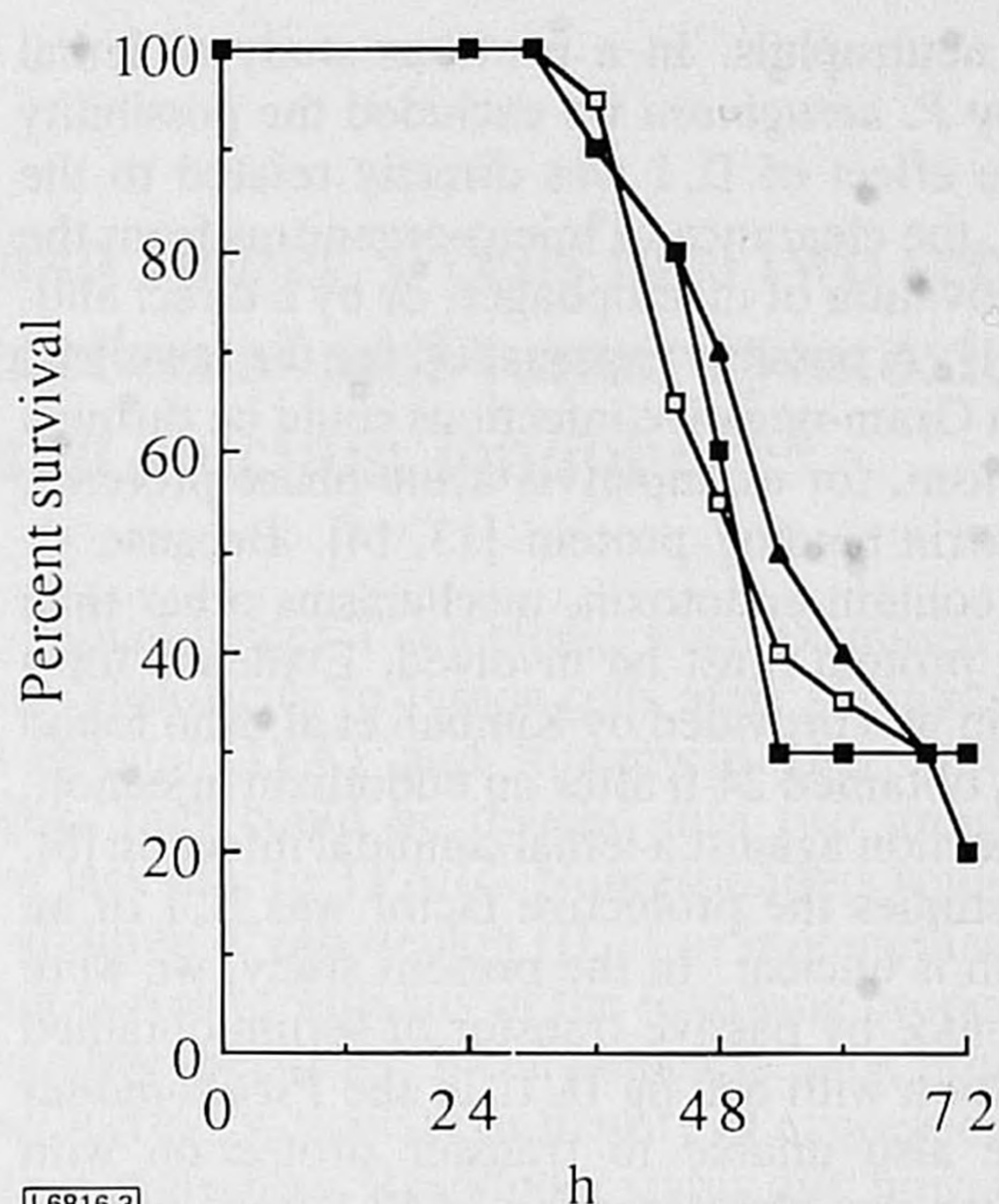
Figure 3. Passive transfer of serum. Serum from mice that received 800 ng IL 1 \beta or saline 24 h before was injected i.p. into recipient mice that were infected with 3 \times 10^5 cfu of C. albicans . The mice were injected with the serum either shortly before the infection (■; n = 10 ) or 24 h after infection (▲; n = 10 ). The survival of these mice does not differ from the controls (□; n = 20 ).
