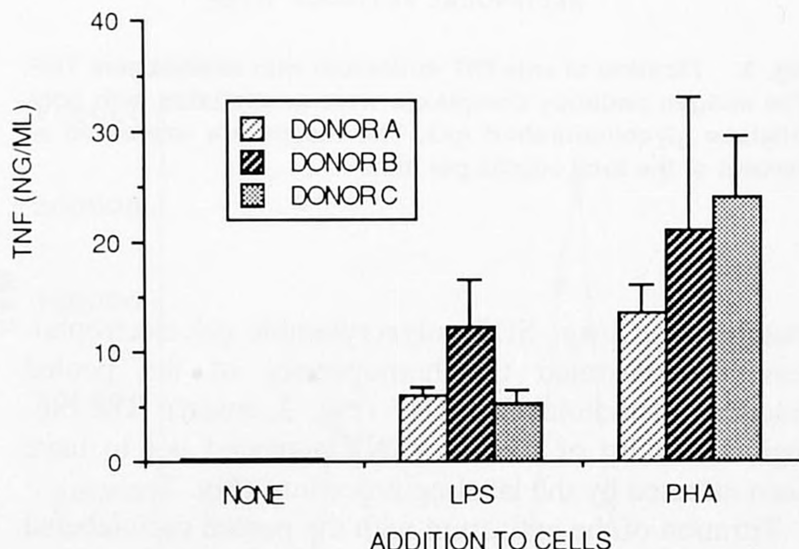
Fig. 7. The consistency of TNF production in vitro; 2.5 \times 10^6 mononuclear cells of 3 different donors were isolated and cultured on three different days. The cells were cultured for 24 h in medium alone, in the presence of 1 ng LPS/ml or PHA 30 \mu g/ml. Supernatants and cell lysates were collected and assayed. Results show the mean and standard deviation on three different days.
