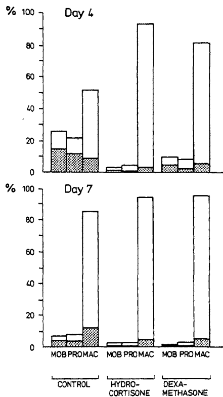
Fig. 4. Differentiation (open bars) and 1-h ^3\text{H} -thymidine labeling (stippled bars) in bone marrow colonies cultured for 4 and 7 days in the presence of 10^{-2} mg/ml hydrocortisone or dexamethasone in Leighton tubes with a coverslip. The bone marrow originated from SPF mice. mob = monoblasts, pro = promonocytes, mac = macrophages.
