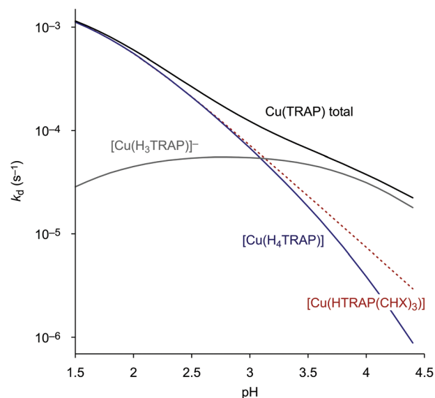
Fig. 2 Contributions of the spontaneous dissociation of the different \text{Cu}(\text{TRAP}) complexes to the overall, pH-dependent reaction rate. In this pH range, the curve for [\text{Cu}(\text{HTRAP}(\text{CHX})_3)] (dotted line) is equivalent to the overall rate for \text{Cu}(\text{TRAP}(\text{CHX})_3) (see Fig. 1), as it is the only contributing species.
