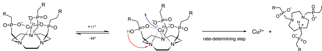
Scheme 3 Proposed mechanism for the proton-assisted dissociation of \text{Cu}^{\text{II}} -TRAP complexes. The colored arrows indicate the structural rearrangements occurring during the rate-determining step. The driving force of the entire reaction is a practically irreversible complexation of \text{Cu}^{\text{II}} by an excess scavenger ligand (not shown).
