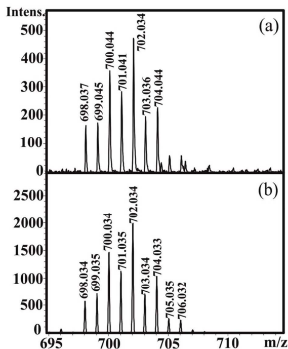
Fig.3. ESI MS spectra recorded in the cadmium(II)–ACSSACS-NH 2 system at pH 7.3 (a) and calculated spectra for the species [CdLCl] − = [Cd(C 18 H 31 N 7 O 9 S 2 )Cl] − (b).
