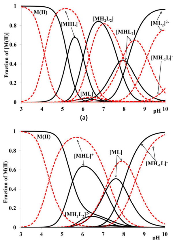
Fig.4. Concentration distribution curves of the complexes formed in the zinc(II) (solid lines) and cadmium(II) (dashed lines)–ACSSACS-NH 2 system at 1:3 ratio (a) and 1:1 ratio (b) (c L = 2 mM)
