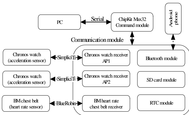
Fig. 2. Activity monitoring system.
