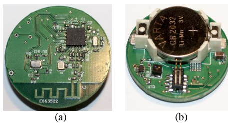
Fig. 3. Acceleration sensor tag.
