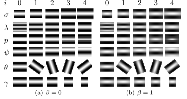
Figure 4: Templates based on various parametrizations of the function H(\sigma, \theta, \lambda, \gamma, q, \beta) . In both cases, the settings \sigma = 10 , \lambda = 16 , \theta = 0 , \gamma = 0.7 , q = 1 are varied by changing one of the parameters: \sigma_i = 8 + i , \lambda_i = 8 + 2i , p_i = 1 - i^{-2} , \psi_i = i\frac{\pi}{5} , \theta_i = i\frac{\pi}{5} , \gamma = 0.7 + 0.2i
