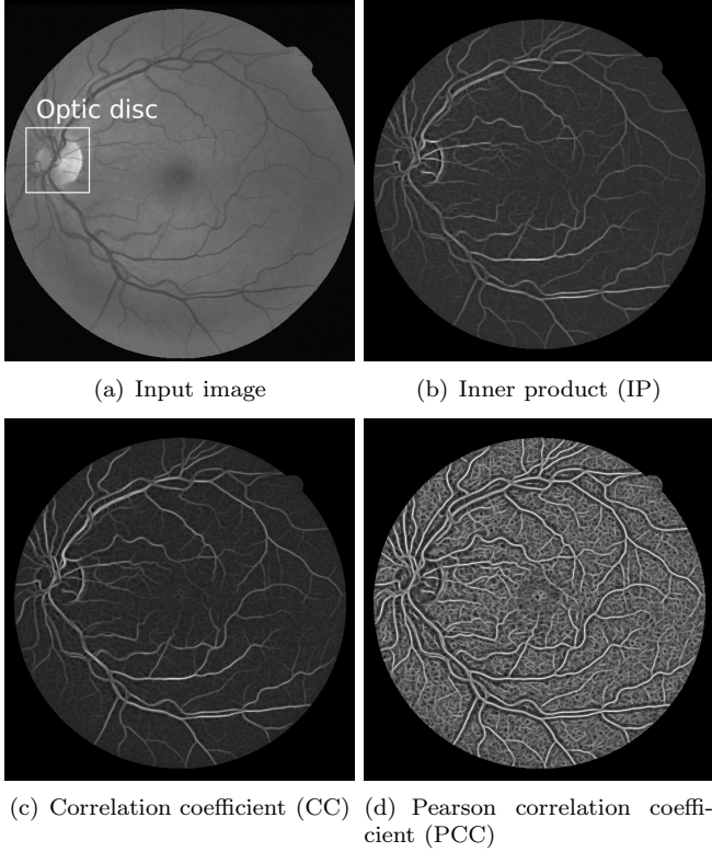
Figure 5: The extended green channel image I_G and the result of template matching with various similarity functions for the parameter setting \sigma = 3 , \lambda = 8 , \psi = \pi , \gamma = 0.5 , \theta \in \{0, \pi/30, \dots, \pi - \pi/30\}
