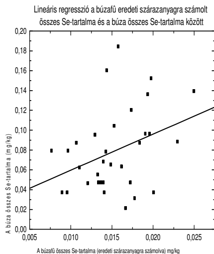
Figure 2: Correlation between the total Se content related to original dry matter of the wheat grass and the total Se content of the wheat
