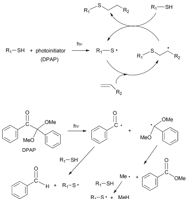
Scheme 1 Sequential thiol-addition and hydrogen abstraction steps during a thiol-ene coupling, and the mechanism for the initiation with the cleavable photoinitiator 2,2-dimethoxy-2-phenylacetophenone (DPAP).
