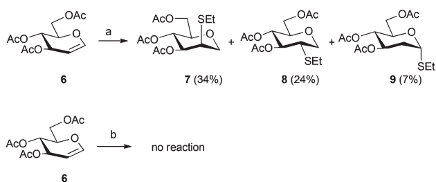
Scheme 3 Reagents and conditions: (a) 15 equiv. of EtSH, toluene, 3 \times 15 min irradiation, 3 \times 0.1 equiv. of DPAP; (b) 50 equiv. of PhSH toluene, 6 \times 15 min irradiation, 6 \times 0.1 equiv. of DPAP.
