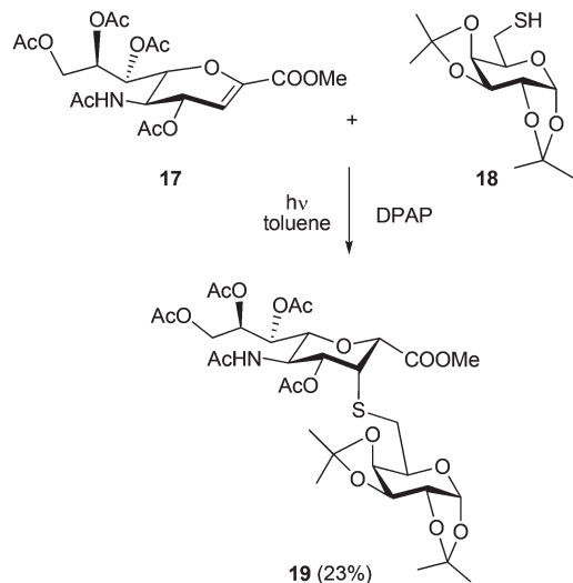
Scheme 4 Reagents and conditions: 2 equiv. of 18, 5 × 15 min irradiation, 5 × 0.1 equiv. of DPAP, 23% for 19; unreacted 17 was recovered in 35% yield.
