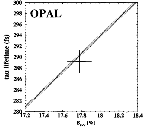
Fig. 3. The OPAL \tau lifetime measurement is plotted against the OPAL measurement of the \tau electronic branching ratio, B_{\text{evv}} . The straight line shows the prediction assuming lepton universality, and the dotted lines reflect the uncertainty associated with the \tau mass.
