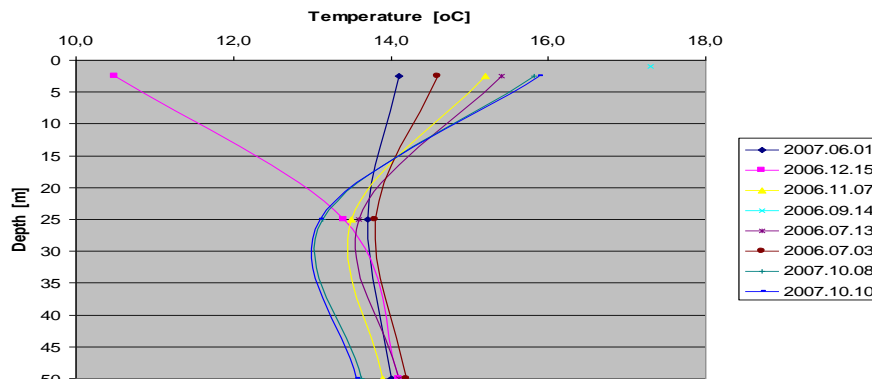
Figure 7. Temperature gradient
