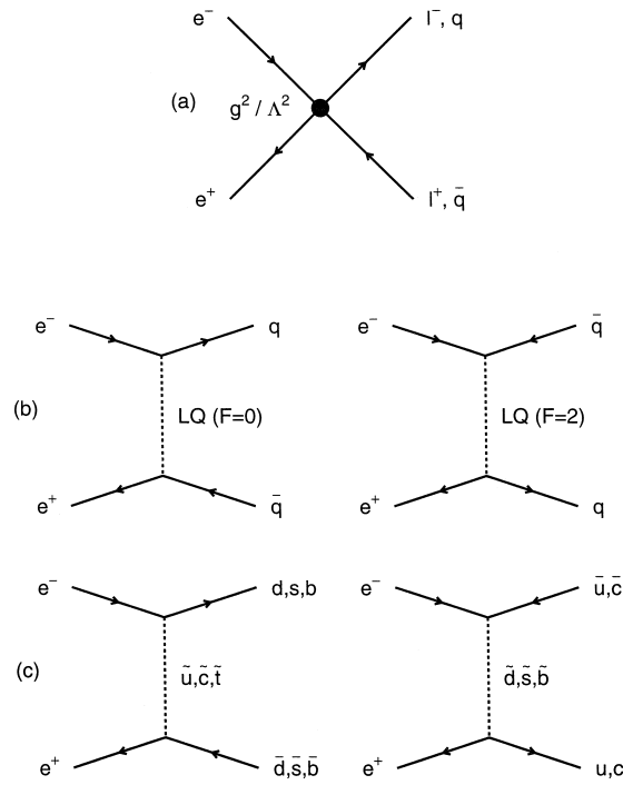
Fig. 1. a) Feynman diagram describing the contact interactions; (b) Feynman diagrams describing the t -channel exchange, left, and u -channel exchange, right, of leptiquarks with fermion number F = L + 3B ; (c) Feynman diagrams describing the t -channel exchange, left, and u -channel exchange, right, of scalar quarks.
