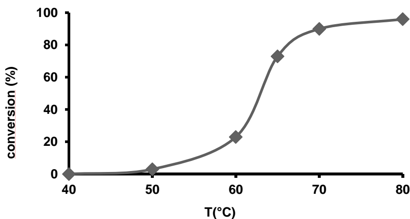
Figure 5. Isomerization of 1-octen-3-ol catalysed by 1 as a function of temperature. Conditions: 0.01 mmol [RuCl 2 (dmsO) 4 ]; 0.50 mmol HCOONa in 3 mL water; 0.08 mL (0.50 mmol) 1-octen-3-ol in 1 mL toluene, t = 1 h.
