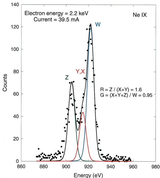
FIG. 3.—Fit to the resonance ( W ; blue line), intercombination ( X, Y ; red line) and forbidden ( Z ; dark green line) lines yields a line ratio R = Z / (X + Y) = 1.6 and G = (X + Y + Z) / W = 0.95 . The collection time was 29 minutes.
