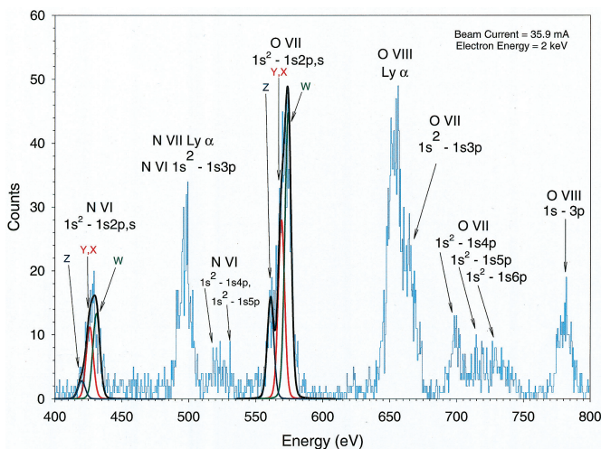
FIG. 1.—Microcalorimeter X-ray spectra from collisionally excited ions of nitrogen and oxygen from the NIST EBIT. The contributions to He-like nitrogen (N VI) and He-like oxygen (O VII) for the forbidden line ( Z ; dark blue line), intercombination line ( Y , X ; red line) and resonance line ( W ; dark green line) are shown. The collection time was \sim 30 minutes.
