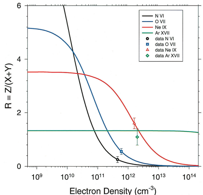
FIG. 6.—Calculated values for R = Z/(X + Y) for N VI (black), O VII (blue line), Ne IX (red line) and Ar XVII (green line). The measured values and their 1\sigma uncertainties are shown by the open data points.
