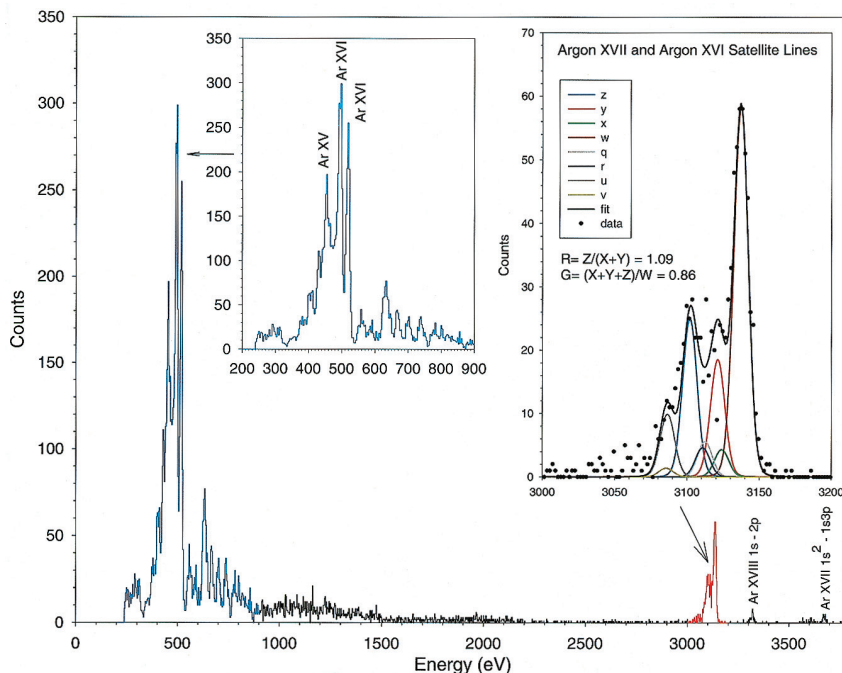
FIG. 4.—Simultaneously observed K and L spectra from Argon. The inset at the upper left shows the richness of the L emission features from argon (blue line). The inset at the right is an expanded view of the He-like complex of Ar XVII (red line) and the additional contributions of the Ar XVI satellite lines. The collection time was 40 minutes.
