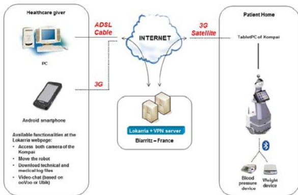
Fig.3. Typically architecture for telepresence and assistive robots [9]
