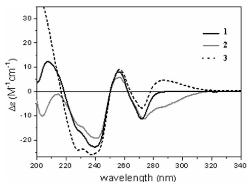
Figure 4. Experimental solution ECD profiles of 1-3 in methanol.
