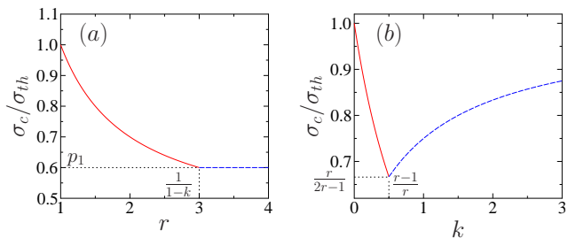
Fig. 2: (Color online) Strength of the two-component system normalized by the breaking threshold \sigma_{th} as a function of (a) the ratio r \equiv E_2/E_1 with fixed k = 2/3 and (b) the ratio k \equiv p_2/p_1 with fixed r = 2 . From both (a) and (b) it can be seen that the single component system is stronger than the two component one.
