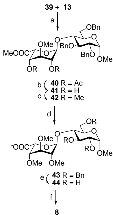
Scheme 7. Synthesis of the GH fragment of idraparinux. Reagents and conditions: (a) \text{CH}_2\text{Cl}_2 , 4 Å Ms, TMSOTf, -20^\circ\text{C} , 30 min (94%); (b) MeOH, NaOMe, rt, 1 h (95%); (c) DMF, \text{Ag}_2\text{O} , MeI, rt, 96 h (76%); (d) 0.1 M NaOH, rt, 24 h (68%); (e) ethanol, Pd(C), \text{H}_2 , rt, 12 h (85%); (f) DMF, \text{SO}_3\cdot\text{py} , 0^\circ\text{C} to rt, 5 h (94%).
