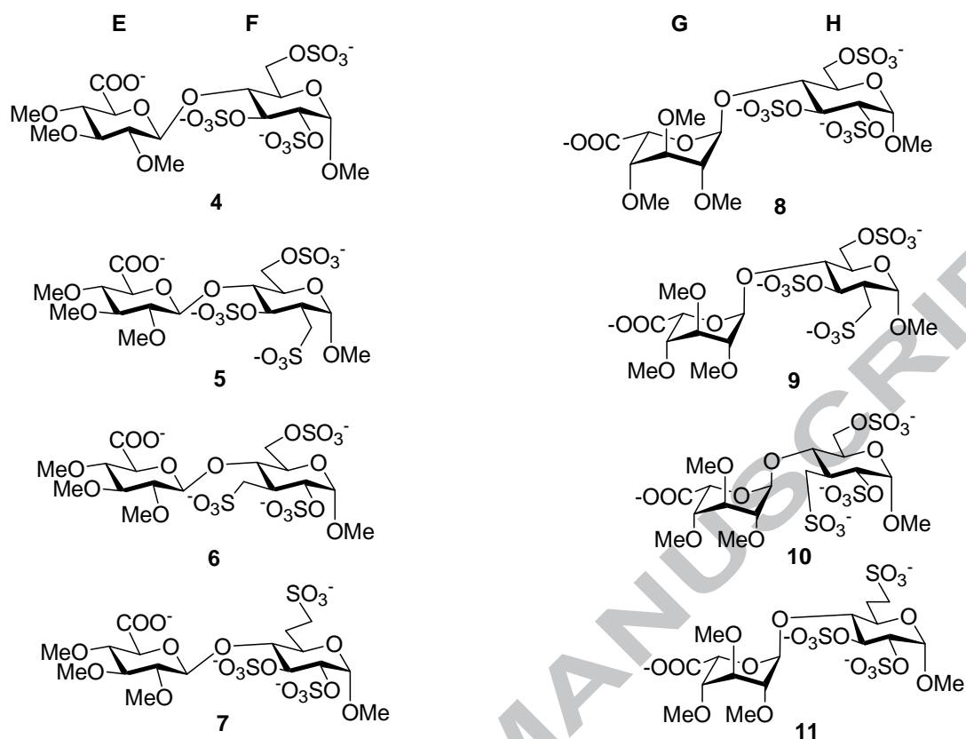
Figure 2. Structures of the EF and the GH fragments of idraparinux ( 4 and 8 ) and their isosteric sulfonic acid derivatives ( 5-7 and 9-11 ).
