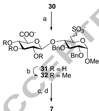
Scheme 5. Synthesis of the 6-deoxy-6-sulfonatomethyl analogue of the EF fragment of idraparinux by selective oxidation. Reagents and conditions: (a) sat NaHCO 3 , KBr, NaOCl, TEMPO, 0 °C to rt, 2 h (91%); (b) DMF, NaH, MeI, 0 °C to rt, 2 h (79%); (c) ethanol, Pd(C), H 2 , 10 atm, rt, 12 h (96%); (d) DMF, SO 3 ·py, 0 °C to rt, 5 h (65%).
