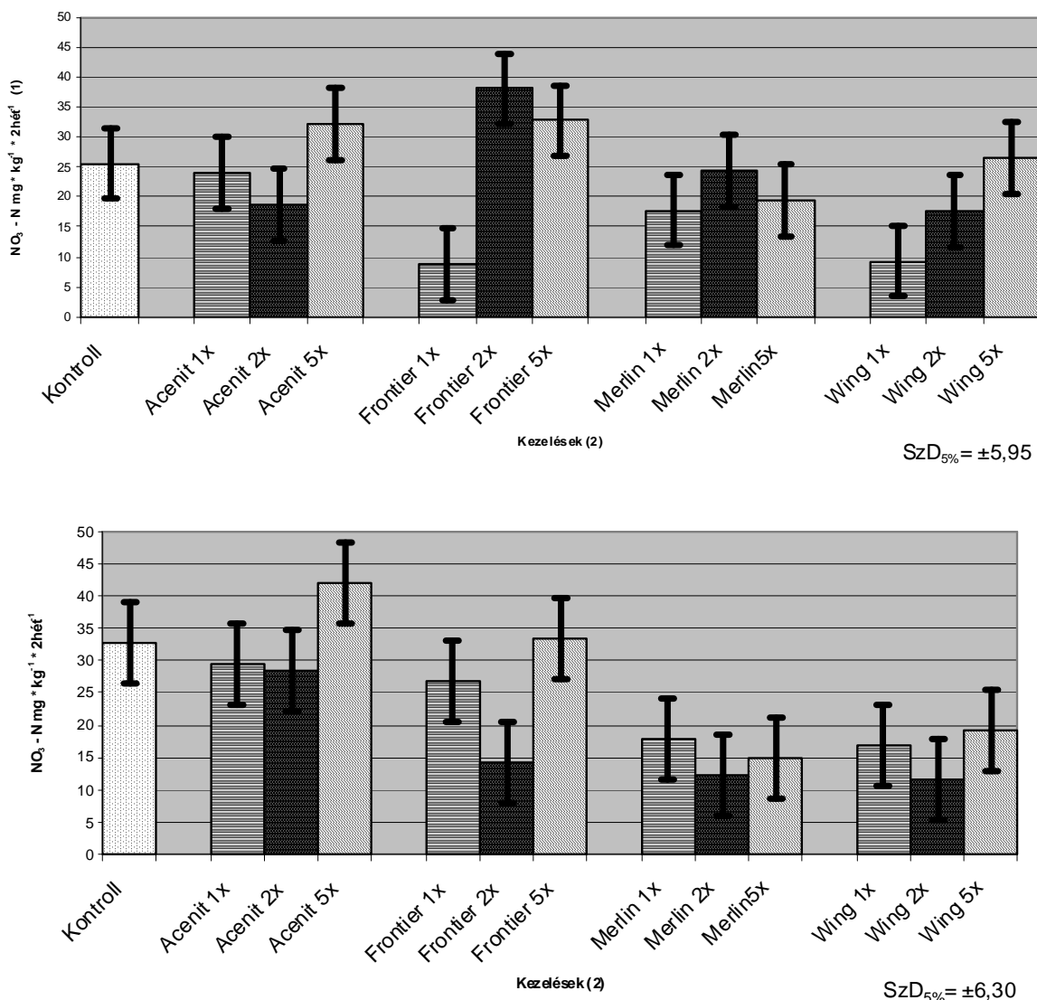
Figure 2.: Effects of herbicides on the \text{NO}_3\text{-N} concentration (1) \text{NO}_3\text{-N} concentration in \text{mg} \cdot \text{kg}^{-1} \cdot 2\text{ weeks}^{-1} (2) herbicides dose
