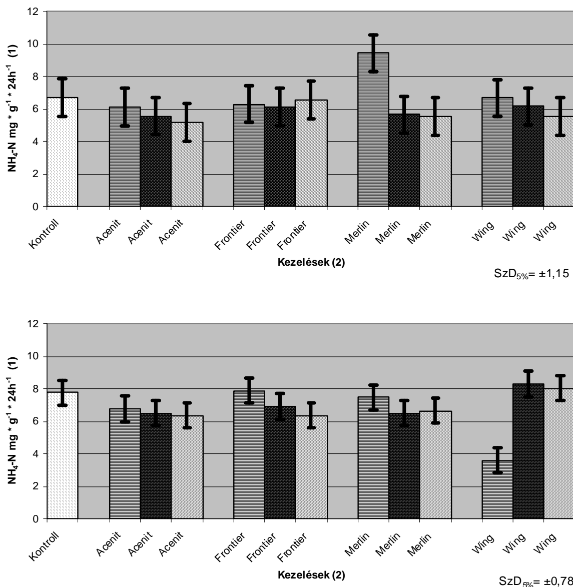
Figure 4: Effects of herbicides on the urease enzyme activity in soil (1) NH 4 -N mg * g soil -1 * 24h -1 (2) herbicides dose
