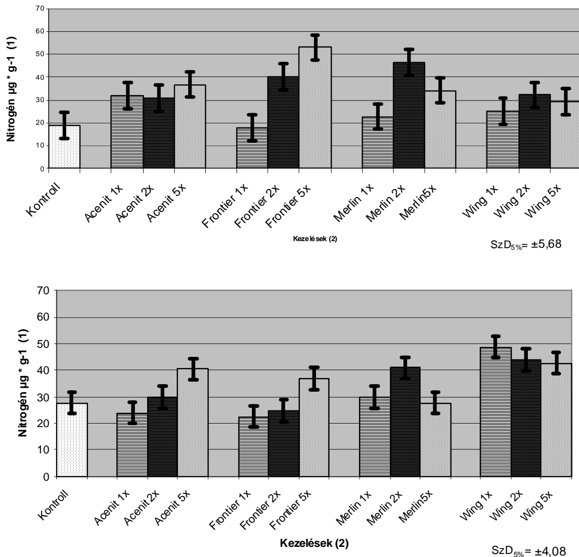
Figure 3: Effects of herbicides on the microbial biomass N (1) \text{N } \mu\text{g} * \text{g soil}^{-1} (2) herbicides dose
