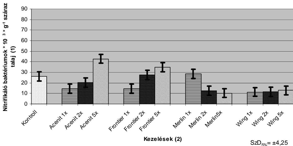
Figure 1.: Effects of herbicides on the number of nitrifying bacteria (1) 10^3 * number of bacteria g soil -1 , (2) herbicides dose
