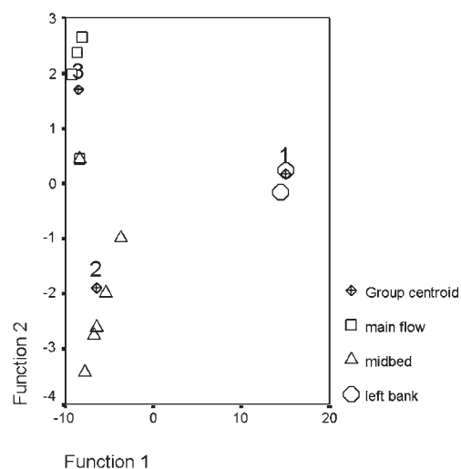
Fig. 2. Classification of sampling sites along the cross-section of River Tisza between Lónya and Tiszamogyorós. All taxa were taken into consideration with chironomids identified to species level. Groups are as follows: 1: left bank, 2: mid-bed, 3: main flow
