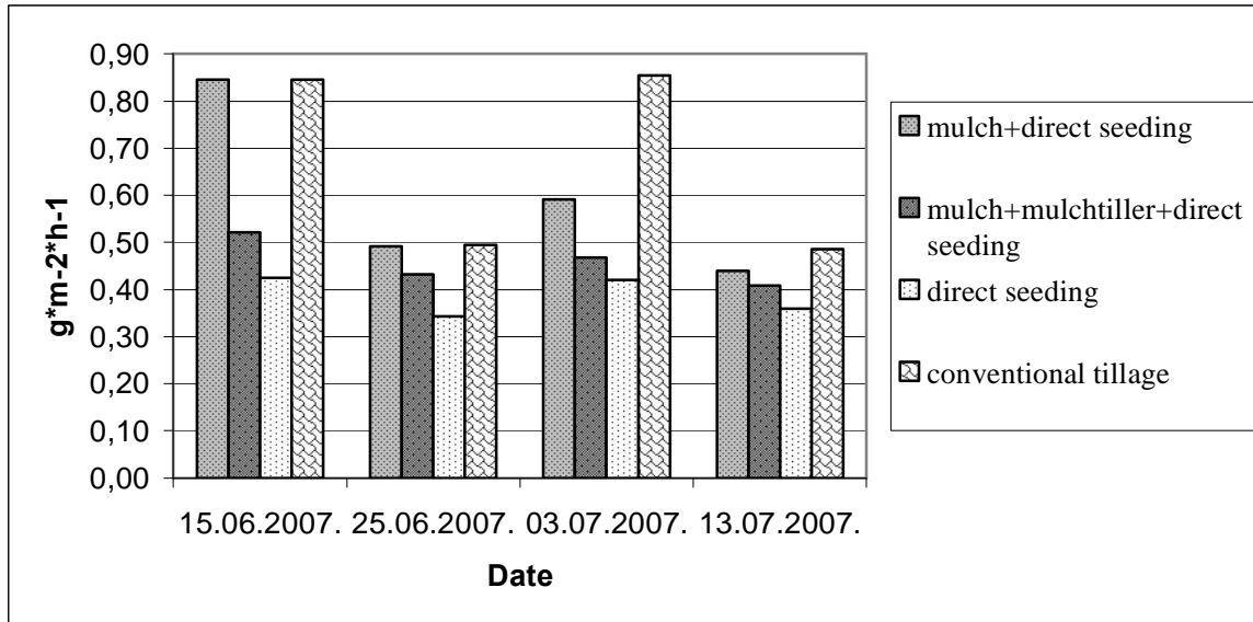
Figure 5.: CO 2 emission on plot I-2
