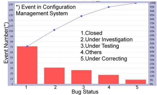
Fig.16 Bug Status at the End of Measurement
