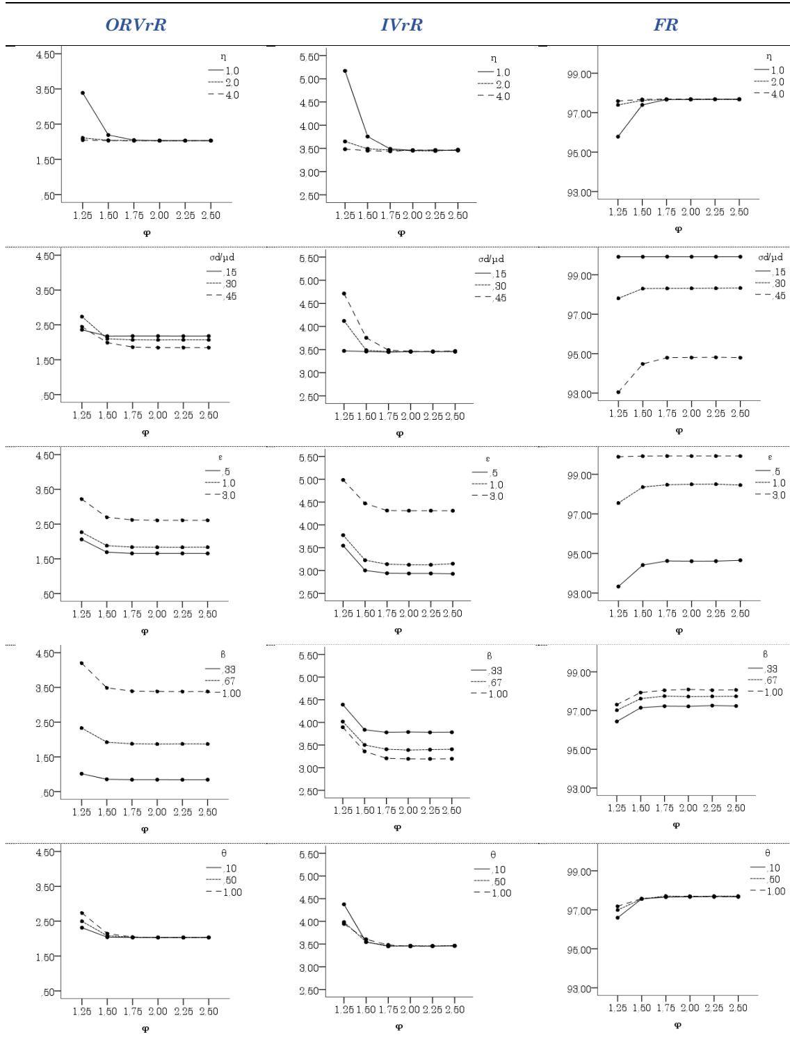
Figure 6. Interaction plots with capacity saturation factor ( \varphi ).
