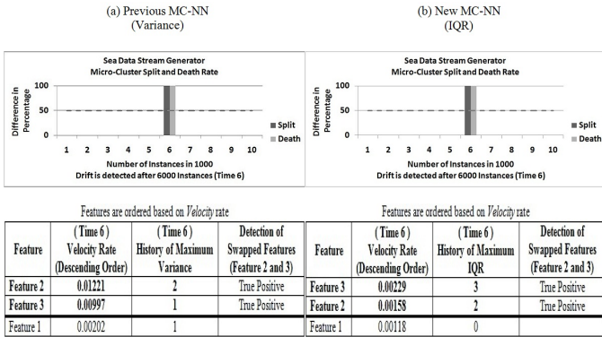
Figure 29: The results of SEA data stream generator with a noise level of 0% for tracking features using Micro-Clusters.
