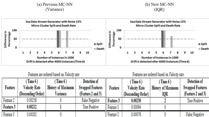
Figure 30: The results of SEA data stream generator with a noise level of 15% for tracking features using Micro-Clusters.
