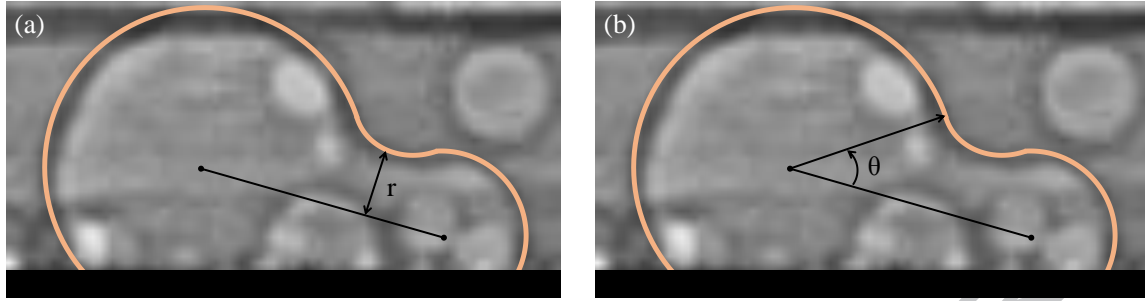
Fig. 6. Schematic of the measurement of (a) bridging neck radius and (b) surface wave propagation angle during coalescence of unequal-sided microbubbles.
