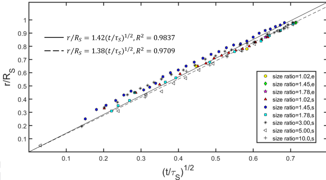
Fig. 7. Time evolution of the bridging neck radius of six coalescence cases with initial radius ratios 1.02 ( 56 \mu\text{m} and 55 \mu\text{m} ), 1.45 ( 42 \mu\text{m} and 29 \mu\text{m} ), 1.78 ( 64 \mu\text{m} and 36 \mu\text{m} ), 3 ( 69 \mu\text{m} and 23 \mu\text{m} ), 5 ( 70 \mu\text{m} and 14 \mu\text{m} ) and 10 ( 70 \mu\text{m} and 7 \mu\text{m} ) obtained from
