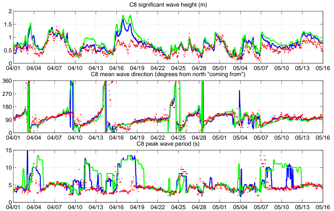
Figure 14 : Model vs. in situ data for the Cluster 8 ADTCP in 9 m depth. Blue line=control model (currents ingested by SWAN), Green line=SWAN model without currents, Red line=in situ data.
