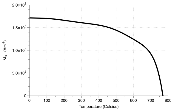
Figure 20. Saturation magnetization vs. temperature for iron.
