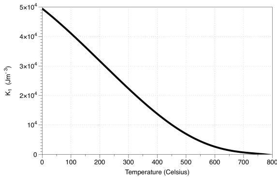
Figure 19. Crystalline anisotropy constant vs. temperature for iron.
