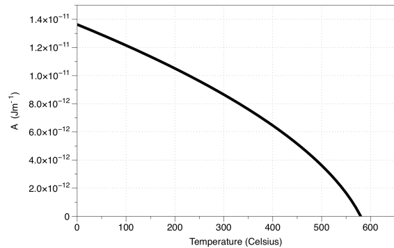
Figure 15. Exchange coupling vs. temperature for magnetite.
