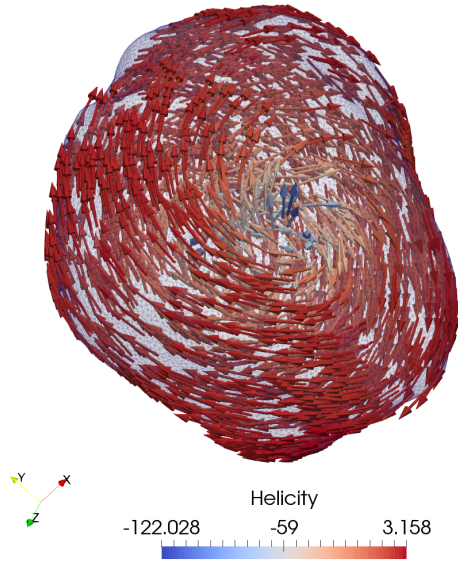
Figure 2. Minimization of an Iron inclusion from a dusty olivine sample at 20 C with random initial magnetization. The shape is approximately a prolate ellipsoid with semi-major axes of 0.134 \mu\text{m} and 0.126 \mu\text{m} , and semi-minor axis of 0.085 \mu\text{m} , with axes aligned along the cardinal directions. The LEM is a single vortex state with core aligned along the semi-minor axis.
