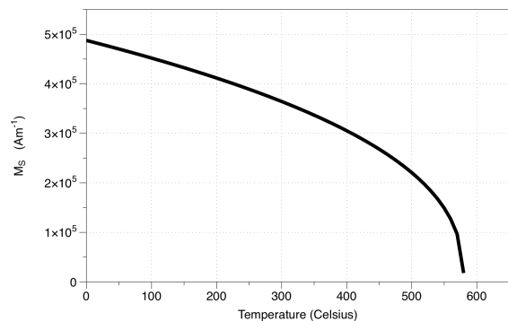
Figure 17. Saturation magnetization vs. temperature for magnetite.
