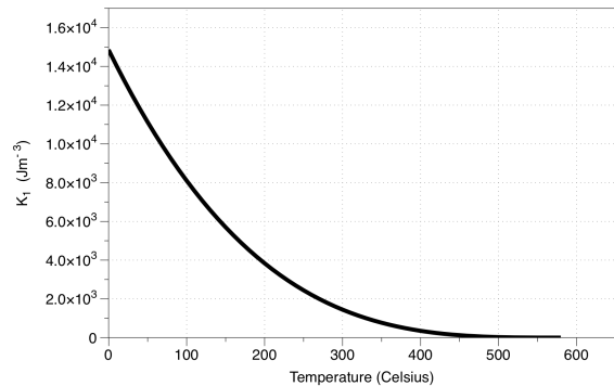
Figure 16. Crystalline anisotropy constant vs. temperature for magnetite.
