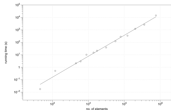
Figure 9. A log-log plot of the time taken for MERRILL to find a Local Energy Minimum of a cube, starting from a random state, versus the number of elements in the mesh.
