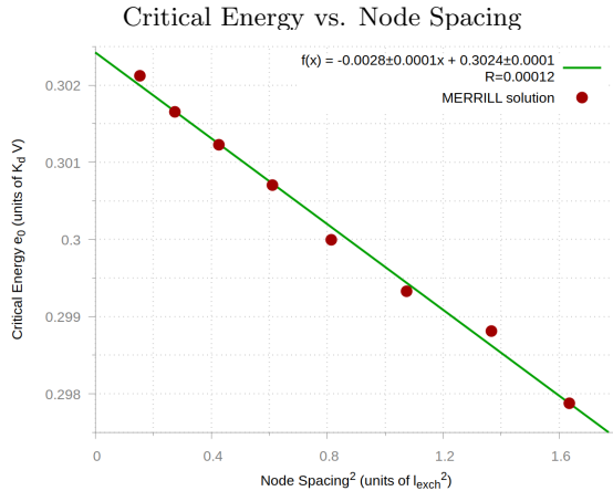
Figure 14. The critical energy versus the node spacing of the mesh, and linear extrapolating the node spacing to 0. This shows the critical energy for an infinitely fine mesh using MERRILL is (0.30242 \pm 0.00008) \times K_d V .
