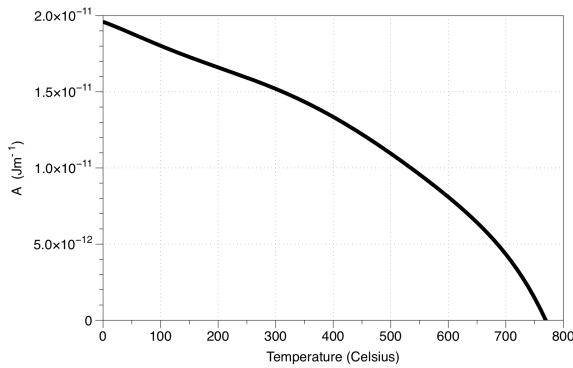
Figure 18. Exchange coupling vs. temperature for iron.
