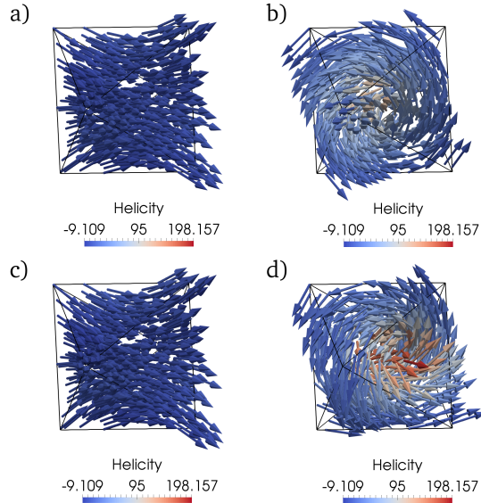
Figure 8. Comparison of upper and lower branch results for a size hysteresis of an octahedral grain of magnetite. The upper branch goes from small to large, and the lower branch goes from large to small. Image a) is the upper branch at 0.13 \mu\text{m} , b) is the lower branch at 0.13 \mu\text{m} , c) is the upper branch at 0.15 \mu\text{m} , and d) is the lower branch at 0.15 \mu\text{m} . The colouring is helicity ( \vec{M} \cdot (\vec{\nabla} \times \vec{M}) ).
