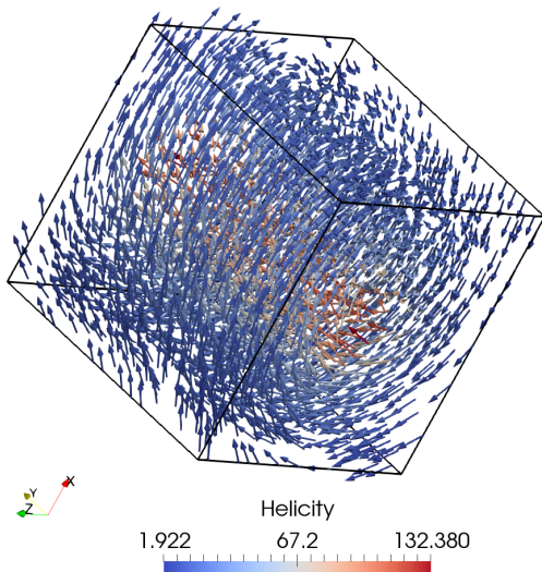
Figure 11. An initial vortex state at edge length 8.45 \times l_{\text{exch}} colored by helicity (\vec{M} \cdot (\nabla \times \vec{M})) .
