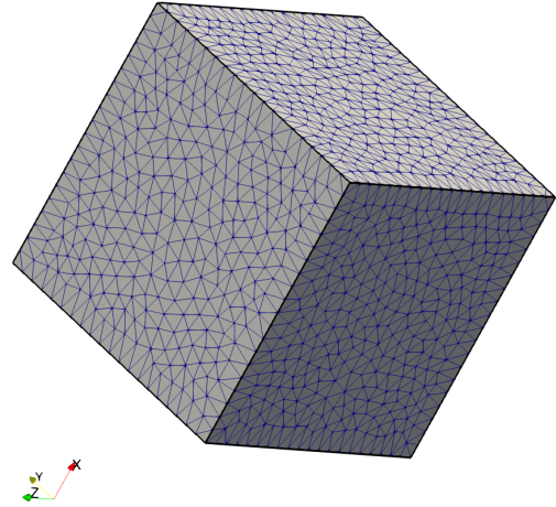
Figure 12. Cube mesh with a node spacing of 0.5 \times l_{\text{exch}} .
