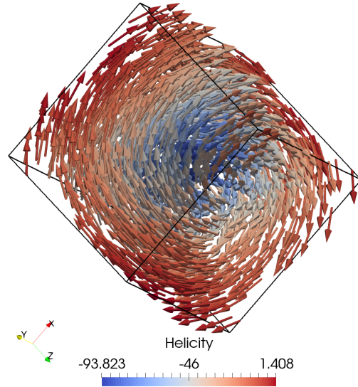
Figure 4. Minimization of a 0.08 \mu\text{m} cube of Magnetite to a vortex state from an initial approximate [111] aligned vortex state, coloured by helicity ( \vec{M} \cdot (\vec{\nabla} \times \vec{M}) ).
