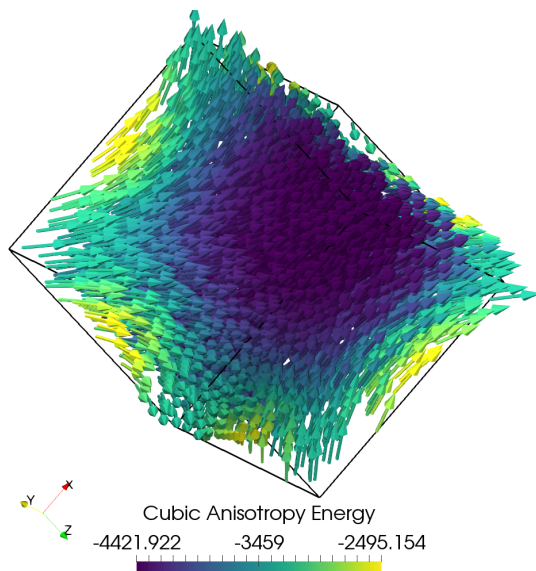
Figure 3. Minimization of a 0.08 \mu\text{m} cube of Magnetite to a flower state from an initial uniform [111] magnetization.
