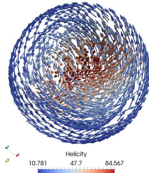
Figure 6. Magnetization of a 0.1 \mu\text{m} sphere of magnetite at |H| = -30 \text{ mT} during a field hysteresis from |H| = -100 \text{ mT} to H = 100 \text{ mT} , coloured by helicity ( \vec{M} \cdot (\vec{\nabla} \times \vec{M}) ).
