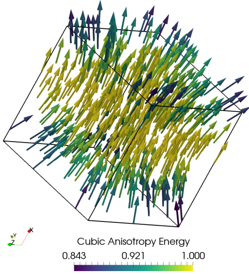
Figure 10. An initial flower solution at edge length 8.45 \times l_{\text{exch}} , colored by the cubic anisotropy energy.
