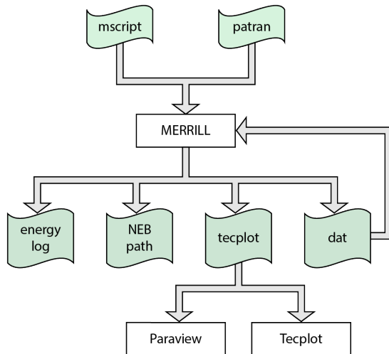
Figure 1. A typical workflow using MERRILL.
