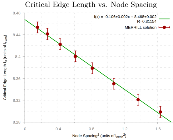
Figure 13. The critical length versus the node spacing of the mesh, and linear fit extrapolating the node spacing to 0. This shows the critical edge length for an infinitely fine mesh using MERRILL is (8.468 \pm 0.002) \times l_{\text{exch}} .
