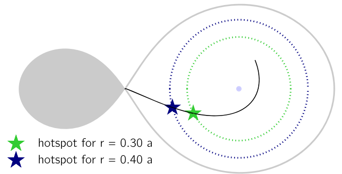
Figure 17. Roche geometry for MLS, with the ballistic trajectory of the accretion stream plotted as a black line. For two different disk radii, the point of collision between the stream and the outer rim of the disk (dashed lines) is shown.
