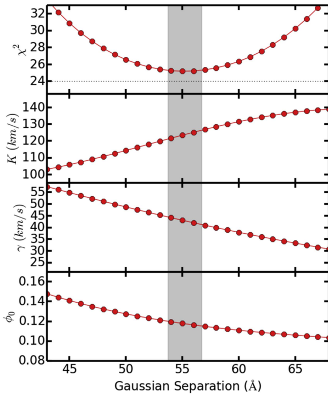
Figure 15. The double-Gaussian method applied to the H_\alpha emission feature, showing that the lowest scatter occurs for a Gaussian separation of 55 \text{ \AA} . The velocity amplitude and center of mass velocity vary slowly with the separation parameter. The time of zero radial velocity shows a significant offset from the time of the photometric eclipse with \phi_0 = 0.12 .
