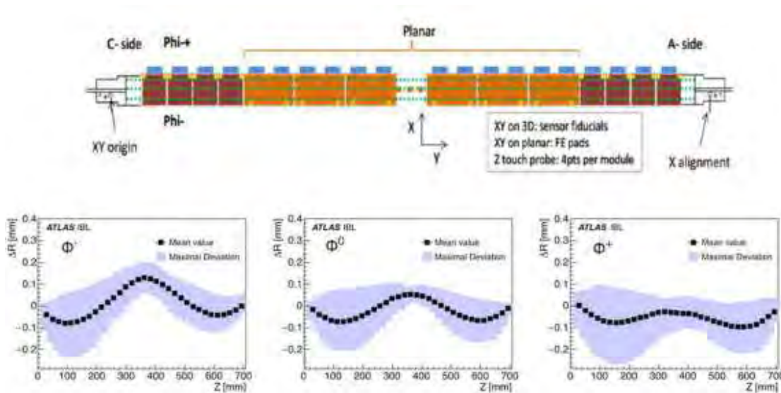
Figure 24. Summary of the planarity, \Delta R , for the 33 production bare staves in three azimuthal positions as defined in the text: (a) \phi^- ; (b) \phi^0 ; and (c) \phi^+ .
