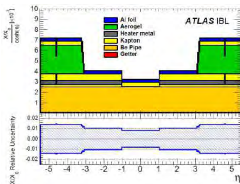
Figure 53. The calculated radiation length X/X_0 of the new beam pipe normalised by \cosh^{-1}(\eta) as a function of \eta . The lower plot shows its relative uncertainty. The Getter (NEG) contribution is small and is not visible.
