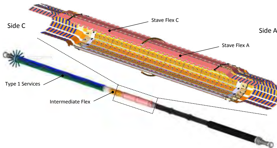
Figure 2. Longitudinal view of the IBL detector and its services. The insert shows an enlarged 3-dimensional view of the detector with its modules arranged cylindrically around the beam pipe.
