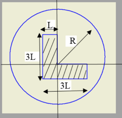
Fig. 4. The die profile (plan view) from round to L-section
