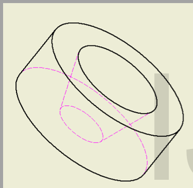
Fig. 6. Streamlined die for extrusion of circular section
