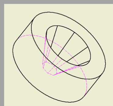
Fig. 11. Streamlined die for extrusion of octagonal section
