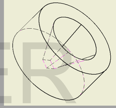
Fig. 8. Streamlined die for extrusion of square section
