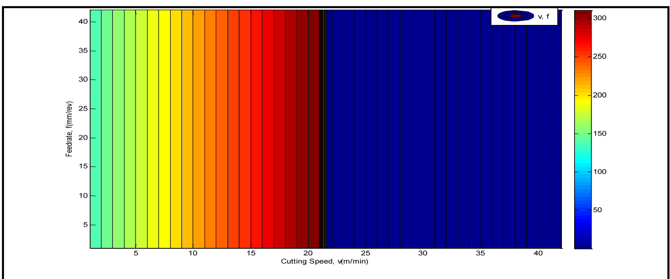
Fig. VIII: Vibration frequency contour plot for cutting Speed vs. feed Rate.
