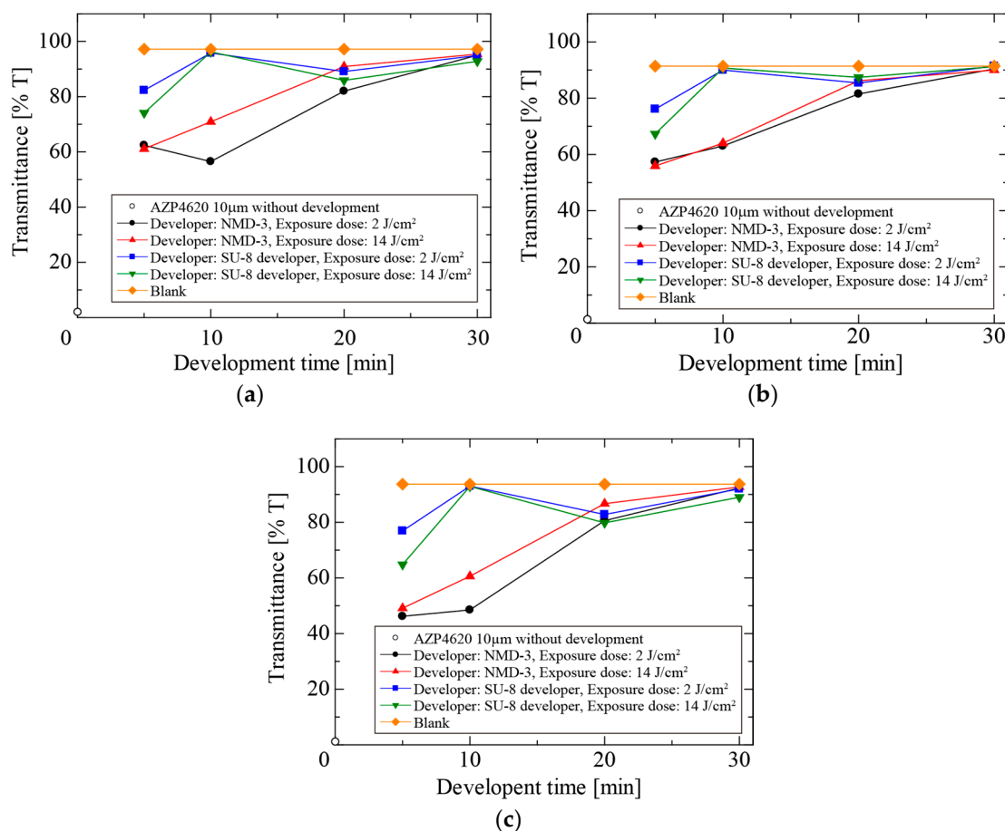
Figure 8. Transmittance vs. development time at (a) g-; (b) h-; and (c) i-line.
