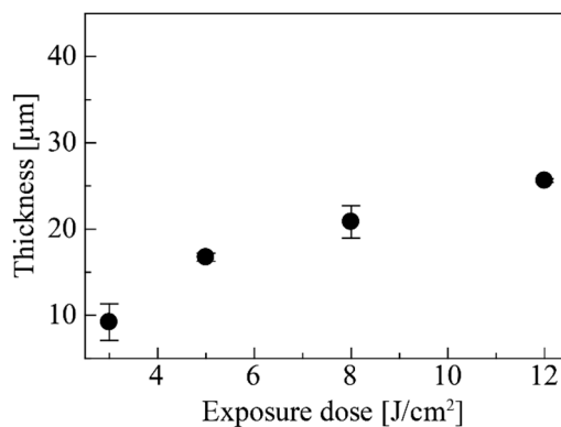
Figure 9. Change in exposed thickness of composite.
