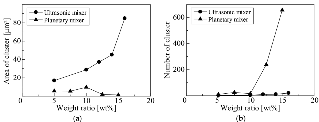
Figure 6. Evaluation of diffusion of magnetic particles in photosensitive composite: (a) Cluster area, and (b) number of clusters with respect to the change in weight ratio of magnetic particles.
