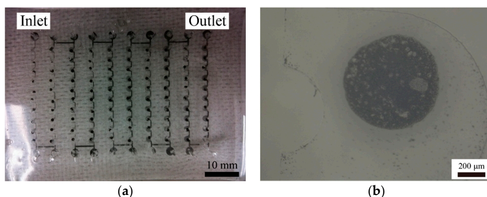
Figure 10. Observation of the fabricated microvalve array device in (a) whole view of the device and (b) enlarged view of microvalve element.
