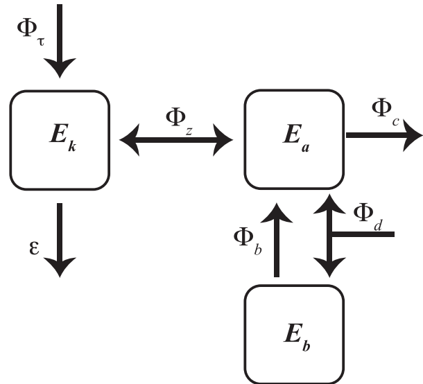
FIG. 1. Energetics of an ocean model, adapted from Hughes et al. (2009). Mechanical energy is defined as the sum of the kinetic energy E_k and the available potential energy E_a . Mechanical forcing \Phi_\tau and conversion of background to available potential energy by surface buoyancy forcing \Phi_b are the primary sources of mechanical energy, with dissipation \varepsilon and parameterized convection \Phi_c acting as sinks of energy. The diffusive contribution \Phi_d can be a source or a sink; \Phi_z is the conversion between E_k and E_a and is closely linked with the overturning circulation.
