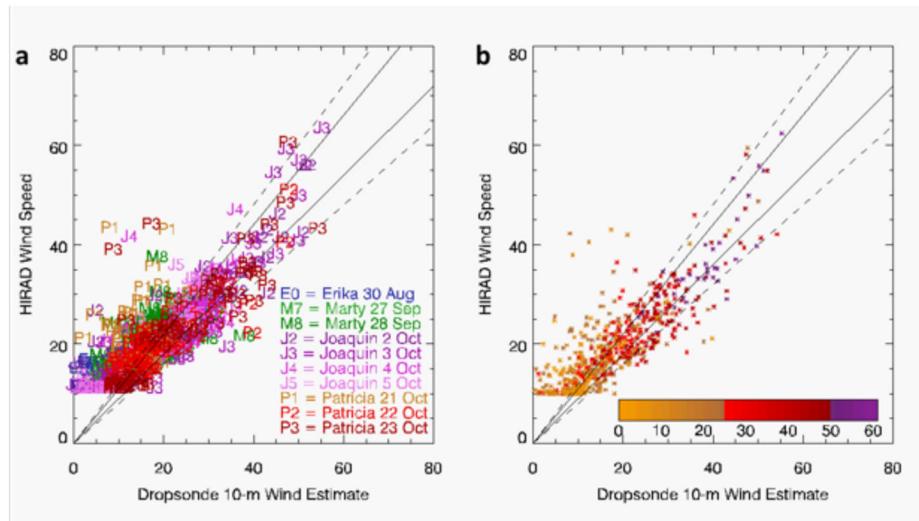
Figure 5. HIRAD retrieved surface wind speed versus dropsonde-estimated surface wind speed. (a) Stratified by flight. (b) Stratified by HIRAD incidence angle. Solid lines mark \pm 10\% agreement; dashed lines mark \pm 20\% agreement.
